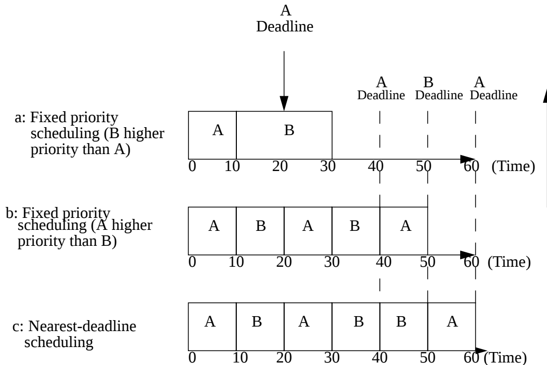
FIGURE 1.4 Concurrency in Real-Time systems
